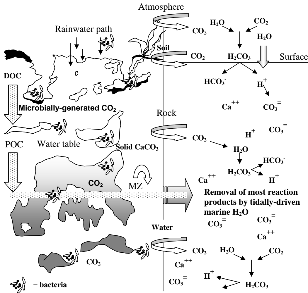
Figure 4. Schematic diagram of some of the chemical activities involved in the dissolution of CaCO 3 and the bacterial sources of CO 2 to drive it. Dark shading represents marine salinity, and White represents freshwater. MZ is the mixing zone. The diagram represents a rock column with a vadose and phreatic zone with water, gases, and bacteria.
